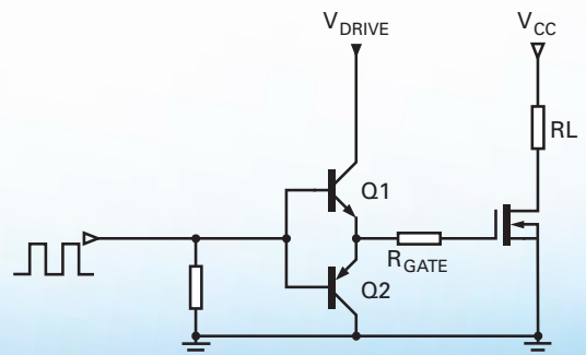
Figure 3. Totem-pole driver stage for power MOSFET
