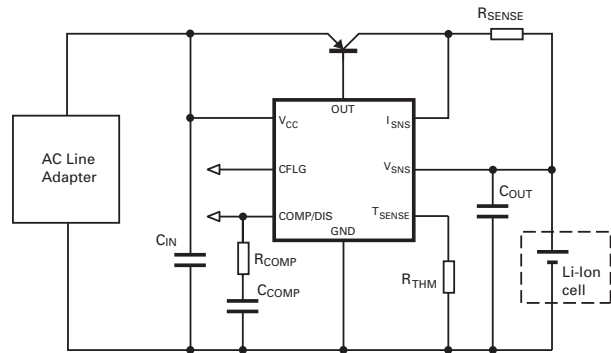
Figure 2. A typical linear charger circuit
